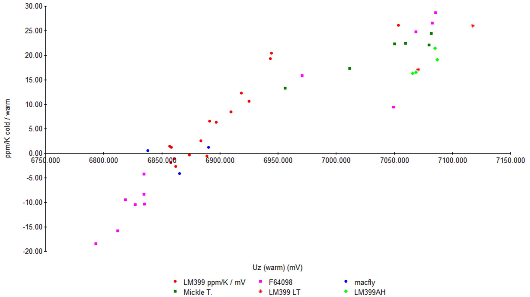
24.02.16 LM399 (un-)heated T.C. over Uz
