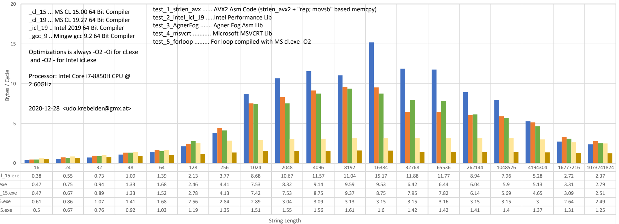
Strcpy Bytes/Clock over Length
