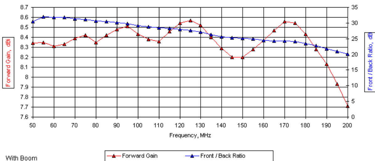
20 Elements/Bay, Alpha = 17°, Tau = 0.9, Psi = 5° Free-Space Forward Gain and 180° Front-to-Back Ratio
