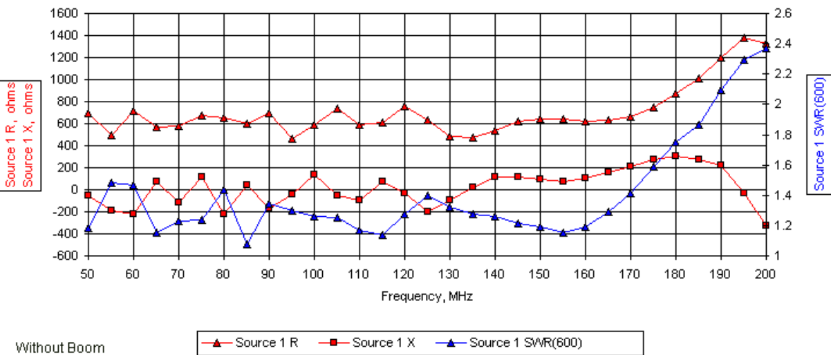
20 Elements/Bay, Alpha = 17°, Tau = 0.9, Psi = 25° Resistance, Reactance, and 600-Ohm SWR
