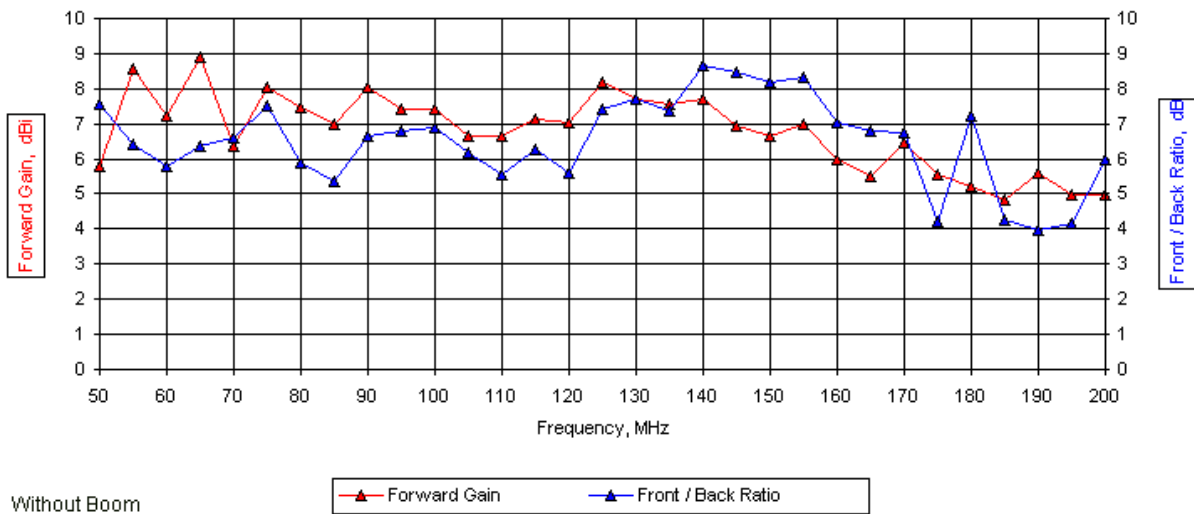
20 Elements/Bay, Alpha = 17°, Tau = 0.9, Psi = 25° Free-Space Forward Gain and 180° Front-to-Back Ratio
