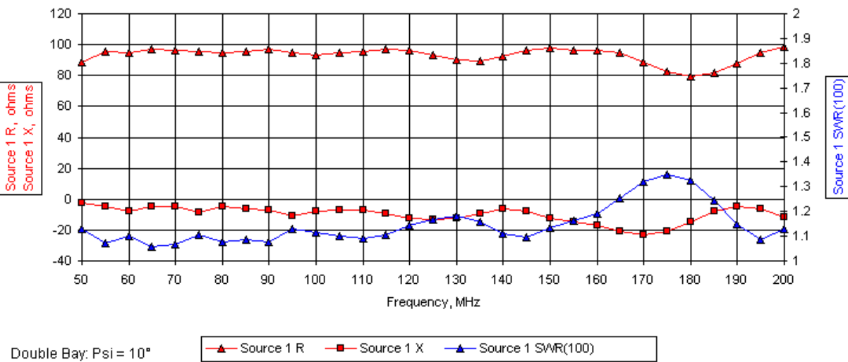
20-Element LPDA, Alpha' = 17°, Tau = 0.9, Sigma = 0.167 Resistance, Reactance, and 100-Ohm SWR
