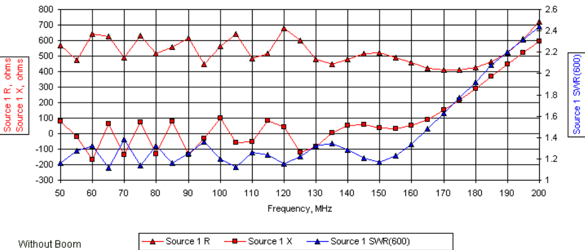
20 Elements/Bay, Alpha = 17°, Tau = 0.9, Psi = 10° Resistance, Reactance, and 600-Ohm SWR
