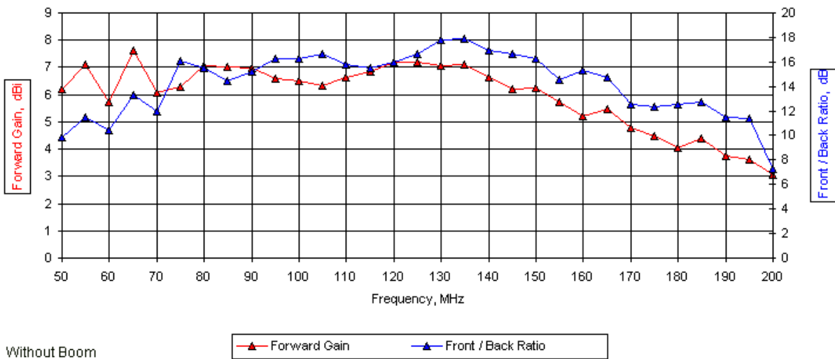
20 Elements/Bay, Alpha = 17°, Tau = 0.9, Psi = 10° Free-Space Forward Gain and 180° Front-to-Back Ratio
