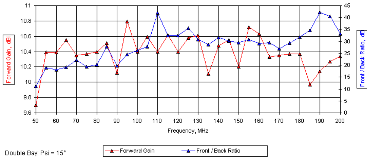
20-Element LPDA, Alpha' = 17°, Tau = 0.9, Sigma = 0.167 Free-Space Forward Gain and 180° Front-to-Back Ratio
