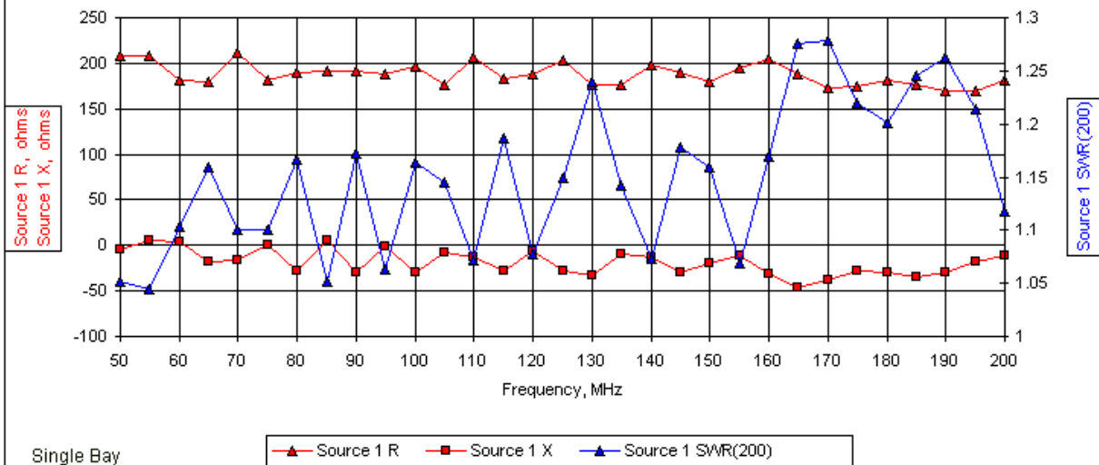
20-Element LPDA, Alpha' = 17°, Tau = 0.9, Sigma = 0.167 Resistance, Reactance, and 200-Ohm SWR
