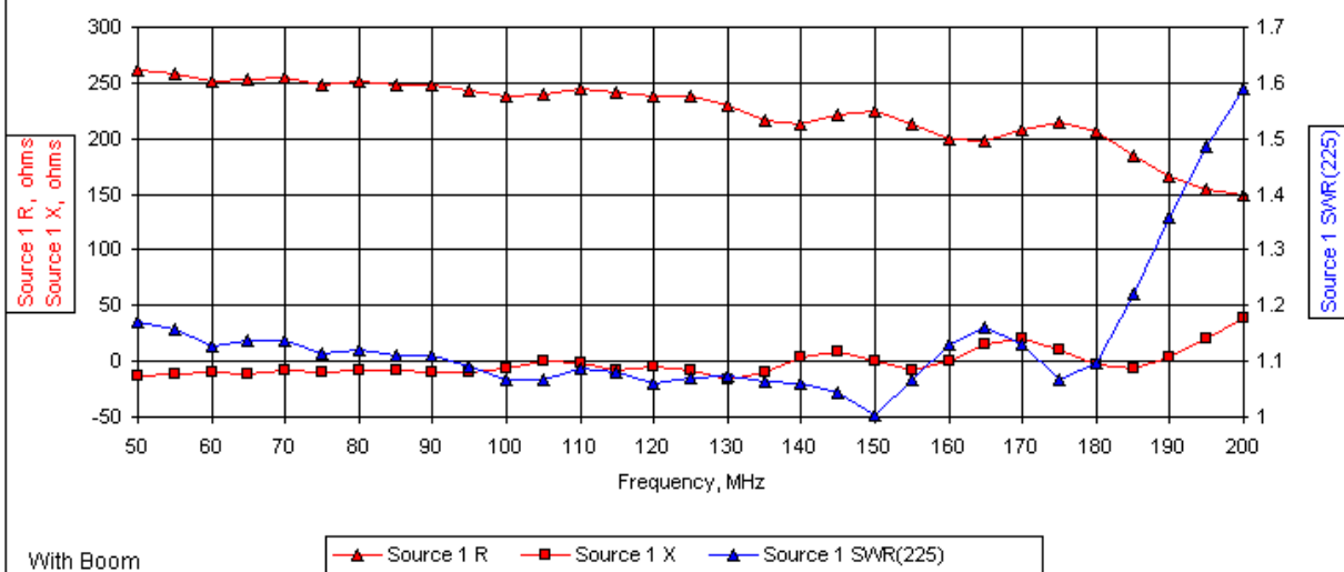
20 Elements/Bay, Alpha = 17°, Tau = 0.9, Psi = 5° Resistance, Reactance, and 225-Ohm SWR
